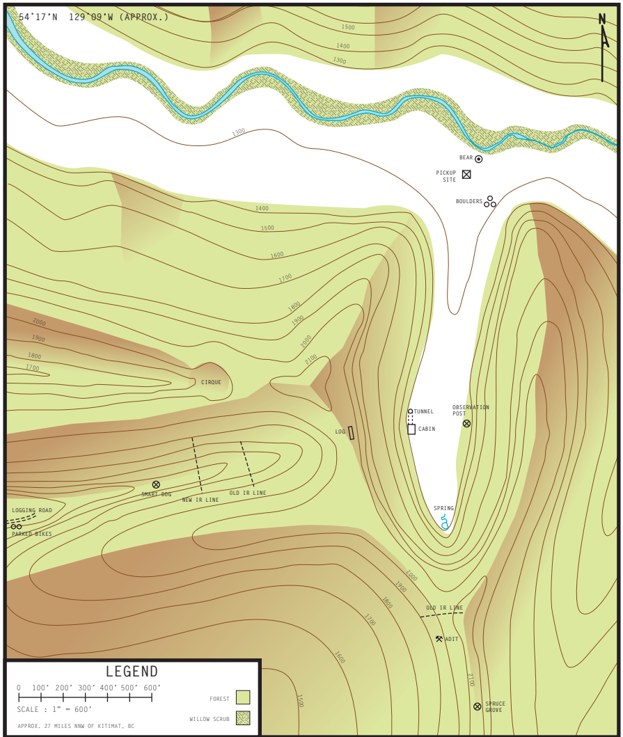
COASTAL RANGE FORMER BRITISH COLUMBIA, CANADA MAY 1, 1927 AD (DETAIL)
